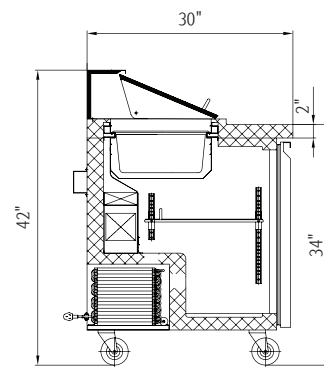
Side Section
